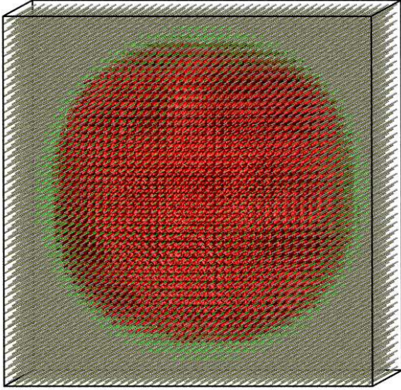
Wavefunctions of highest occupied states
