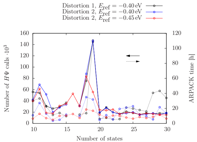
FIG. 2: Number of iterations required to achieve convergence with respect to the number of requested states for a GaAs bulk structure consisting of 1,728 atoms, for which two different distortions are applied to a single Ga atom of the structure.
