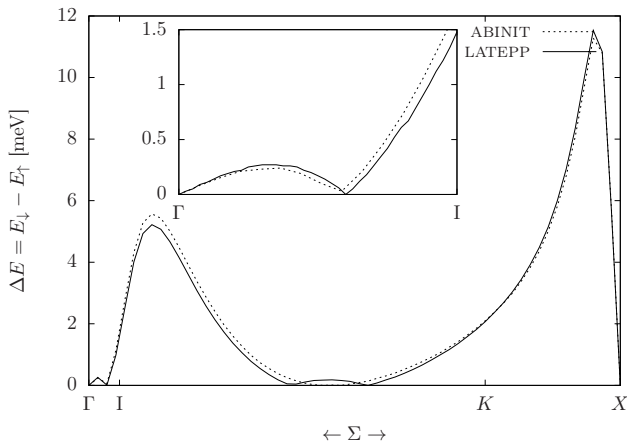
FIG. 16: Spin splitting of the GaAs heavy hole band from \Gamma to X along \Sigma direction. The inset shows a magnified region near the \Gamma point. Results of LATEPP (solid line) are compared to results of ABINIT employing the HGH 56 potentials (dashed line).
