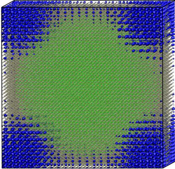
Wavefunctions of lowest unoccupied states
