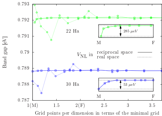
FIG. 3: Convergence of the band gap energy of a bulk GaAs supercell containing eight atoms for two plane wave energy cut-offs (green: 22 Ha, blue: 30 Ha) with respect to the grid size in one dimension in terms of the minimum grid (M); the full grid is indicated by (F). Results are shown for calculations in the reciprocal space basis with the non-local potential being evaluated in real space (dashed line) and reciprocal space (solid line).
