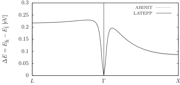
FIG. 13: Lifting of the light/heavy hole degeneracy in GaAs due to spin-orbit interaction. The results of LATEPP (solid line) are compared to a DFT result using ABINIT employing the HGH 56 pseudopotentials (dashed line).
