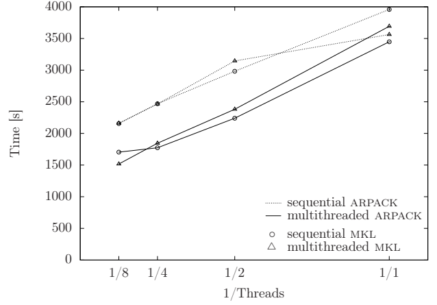
FIG. 8: Total calculation time for a QD structure consisting of 4 \times 4 \times 4 lattice constants containing 512 atoms with respect to the number of threads. Results of four different combinations of libraries utilized in LATEPP are shown.
