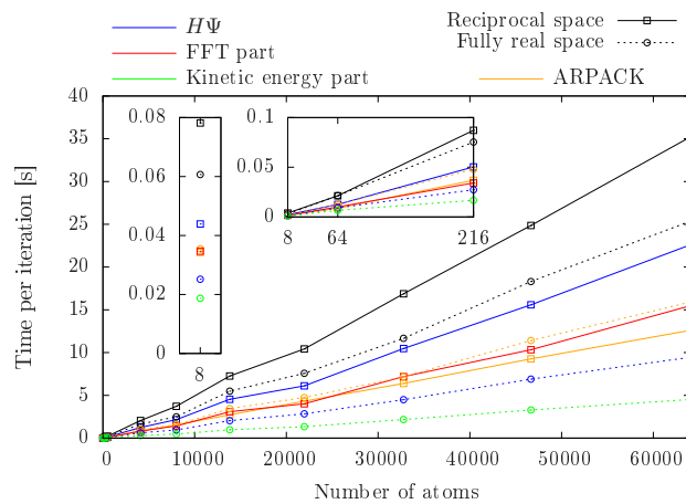
FIG. 10: Time for one iteration (black lines) for bulk GaAs structures with respect to the number of atoms. Results are shown for fully real-space calculations (dashed lines) as well as for calculations in the reciprocal space basis with the non-local potential being evaluated in real space (solid lines). The total time is composed of the time of the H\psi evaluation (blue lines) and the ARPACK routine (orange lines). The treatment in reciprocal space requires FFTs (red line) while a more computationally intensive kinetic energy evaluation (green line) is used in the real space treatment. A minimum grid (see Fig. 3) and 22 Ha cut-off energy for the plane waves are used.
