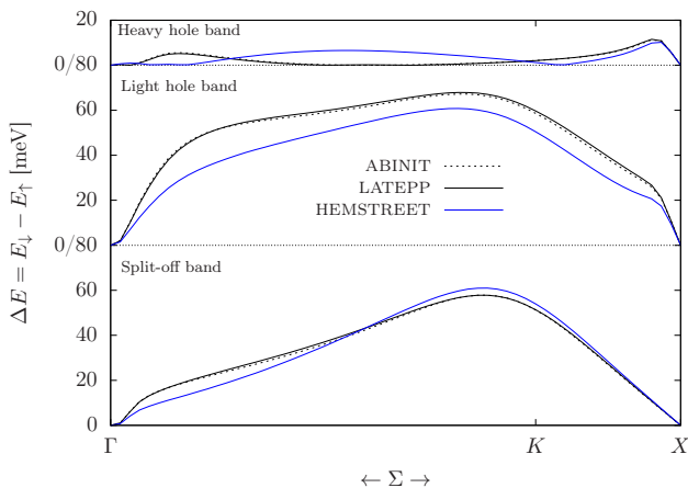
FIG. 17: Spin splitting in the valence bands of GaAs between the \Gamma and X point along the [1\ 1\ 0] direction due to spin-orbit interaction. Results of LATEPP (solid lines) are compared to DFT results using ABINIT employing the HGH 56 potentials (dashed lines). In addition, results with the wrong normalization as given in Refs. 47–49 are shown (blue lines).
