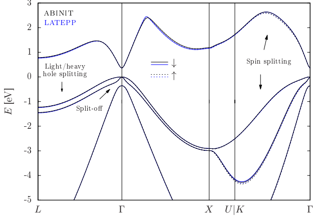
FIG. 12: Electronic band structure of GaAs illustrating the lifting of the degeneracy of the split-off and heavy/light hole band at the \Gamma point as well as the characteristic splitting of the heavy and light hole band approaching the L and X point due to spin-orbit interaction. In addition, the spin splitting of the two spin components (dashed and solid lines) between the X and \Gamma point along [110] can be seen. The results of LATEPP (blue lines) are compared to DFT results using ABINIT employing the HGH 56 pseudopotentials (black lines).
