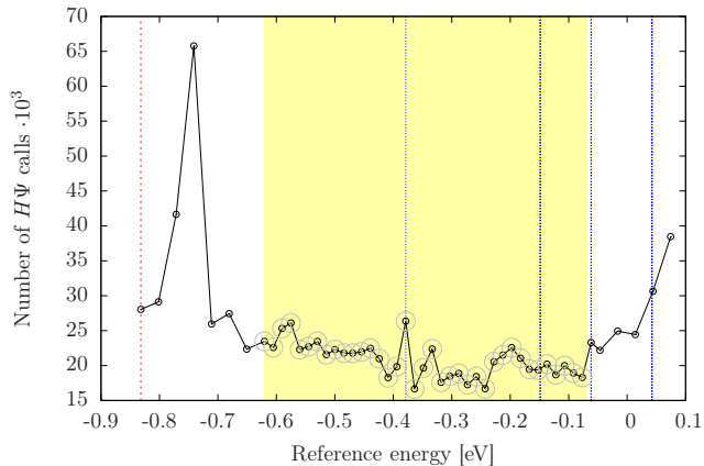
FIG. 1: Number of iterations of the ARPACK solver requesting 14 states with respect to the utilized reference energy. The shaded region marks the range of reference energies for which the same solutions are expected. Data points supplied with a circle identify calculations that indeed contain these solutions. The blue lines correspond to the 4 blocks of eigenvalues of the requested states. The red line corresponds to the middle of the band gap.
