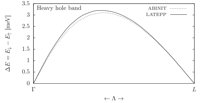
FIG. 15: Spin splitting in the heavy hole band of GaAs between the L and \Gamma point along the \Lambda direction due to spin-orbit interaction. The result of LATEPP (solid line) is compared to the DFT result using ABINIT employing the HGH 56 potentials (dashed line).
