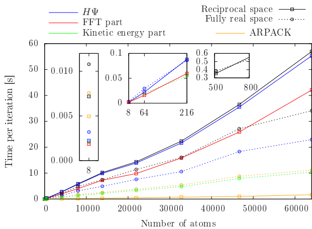
FIG. 11: Time for the first iteration of fully real-space calculations (dashed line) and calculations in the reciprocal space basis with the non-local potential being evaluated in real space (solid line) for different sizes of bulk GaAs structures. The insets show magnified regions of the plot. The contribution of the H\psi evaluation and the ARPACK routine is shown by the blue and orange line respectively. The contributions of the FFT and kinetic energy calculation within the H\psi evaluation are highlighted by red and green colors.
