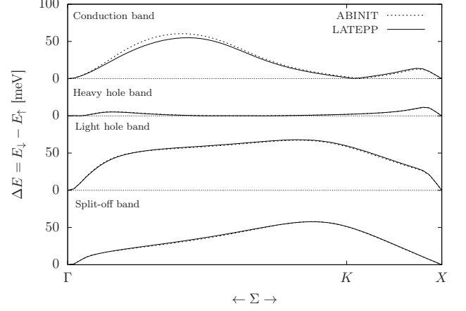
FIG. 14: Spin splitting in the valence and conduction bands of GaAs between the \Gamma and X point along the [110] direction due to spin-orbit interaction. Results of LATEPP (solid lines) are compared to DFT results using ABINIT employing the HGH 56 potentials (dashed lines).
