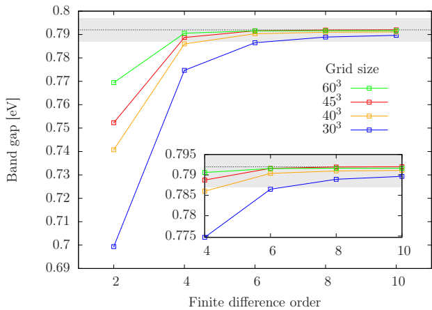
FIG. 5: Convergence of the band gap energy of a bulk GaAs supercell containing eight atoms with respect to the polynomial order of the finite difference scheme in the fully real-space calculations. Results for different grid sizes are shown.
