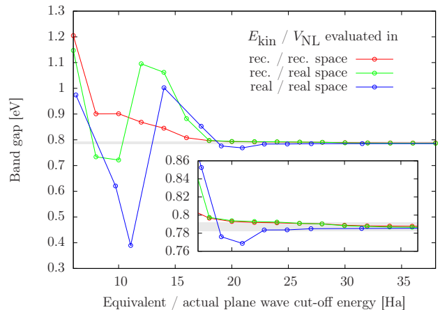
FIG. 4: Convergence of the band gap energy of a bulk GaAs supercell containing eight atoms with respect to the plane wave cut-off energy. For the full real-space calculations the equivalent cut-off energy is calculated according to Eq. (46). The kinetic energy is calculated in real (blue) or reciprocal space (red or green) and the non-local potential in real (blue or green) or reciprocal (red) space.
