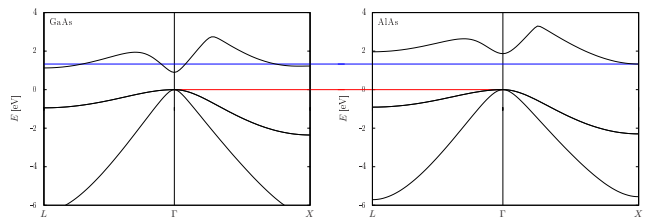
FIG. 6: Excerpt of the electronic band structure of the highest occupied p and the lowest unoccupied s state of GaAs (left) and AlAs (right) bulk structures.
